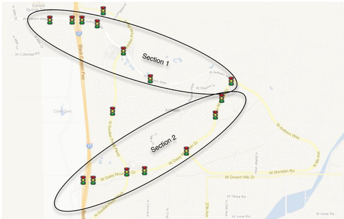
Figure 8 – A MMITSS System Organized into Two Network Sections for Traffic Management
