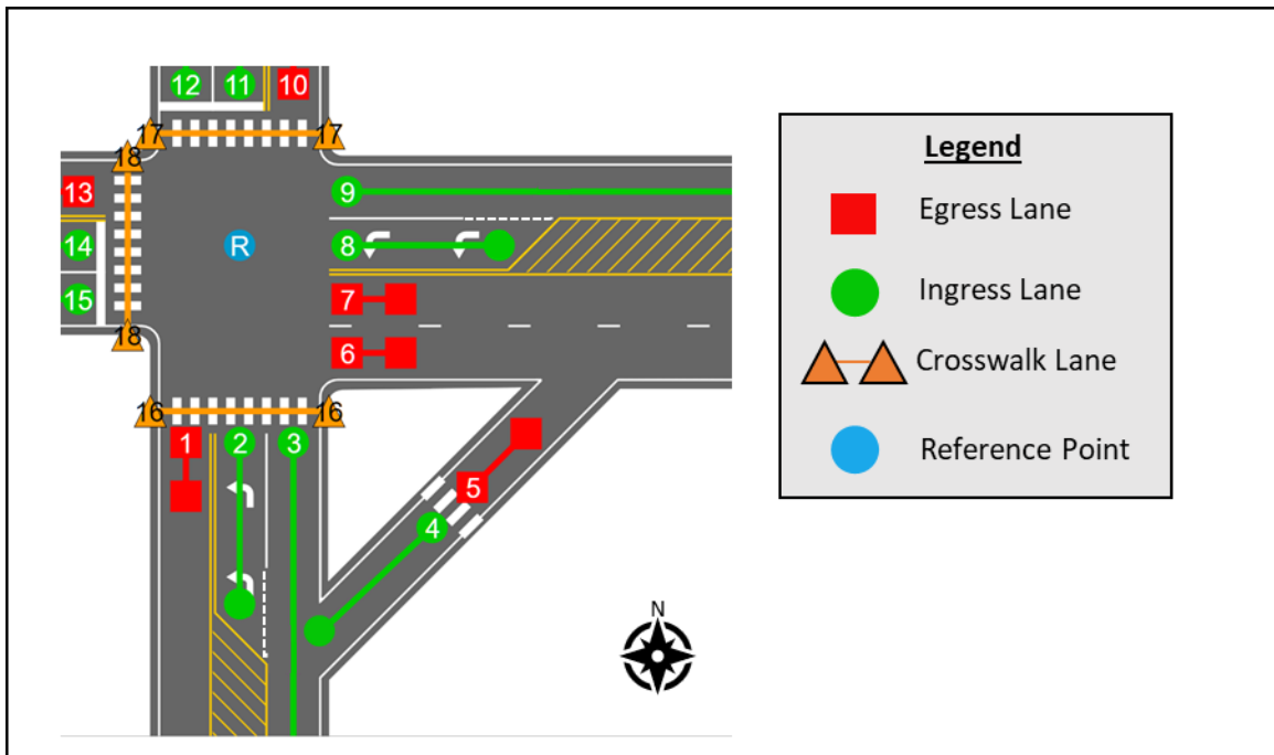
Figure 28: Intersection Turn Lane Node Placement Source: Athey Creek Consultants and Synesis Partners
