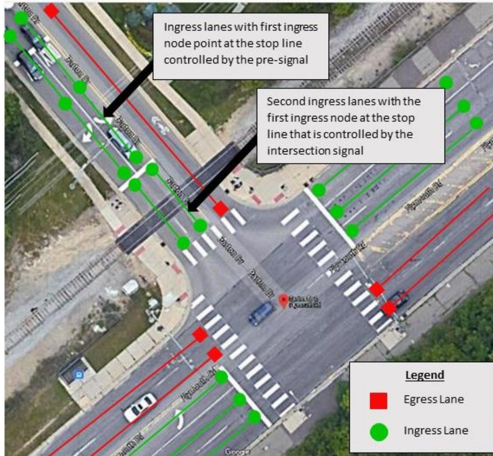
Figure 20: Pre-Signals
