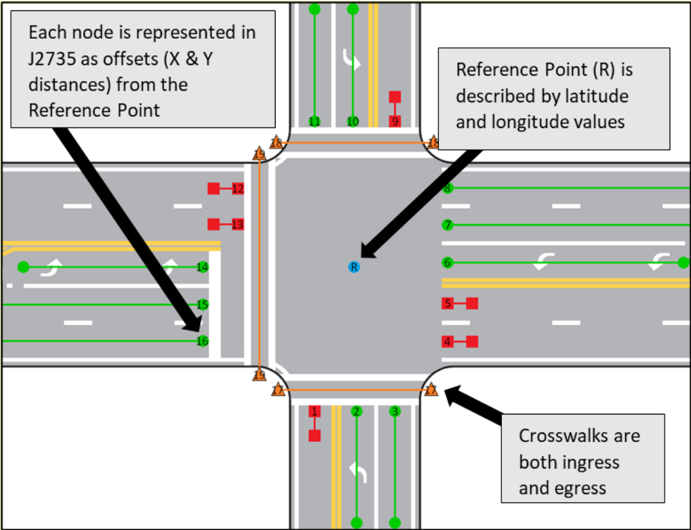
Figure 11: Ingress and egress lane numbering and first node points Source: Athey Creek Consultants and Synesis Partners
