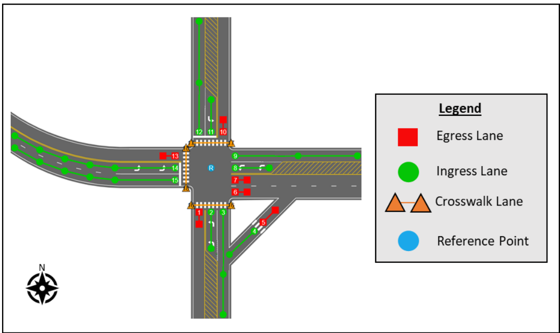
Figure 27: Intersection Lane Nodes
