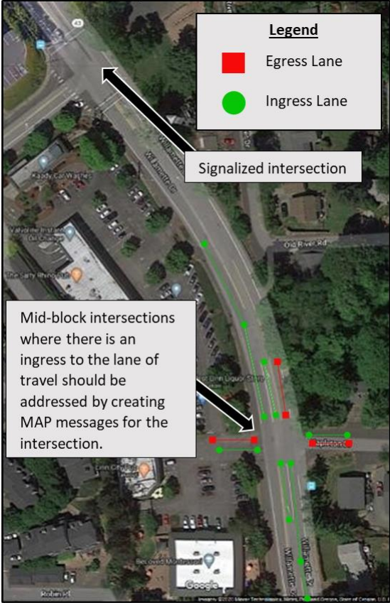
Figure 15: Non-signalized Intersections Map source: Google Maps, Drawing Source: Athey Creek Consultants
