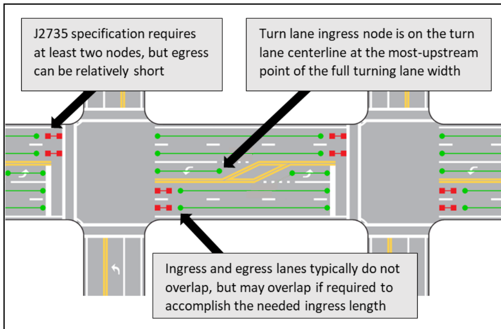
Figure 12: Length of ingress and egress Lane Source: Athey Creek Consultants and Synesis Partners
