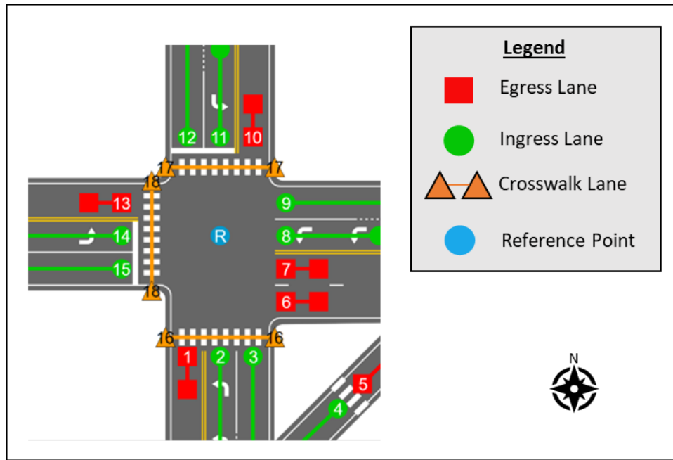
Figure 1: Illustration of example lane ID numbering approach Source: Athey Creek Consultants and Synesis Partners
