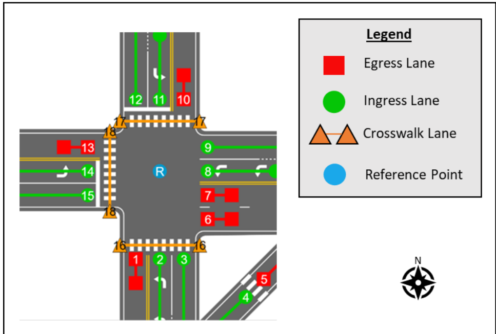
Figure 26: Intersection Lane Numbers
