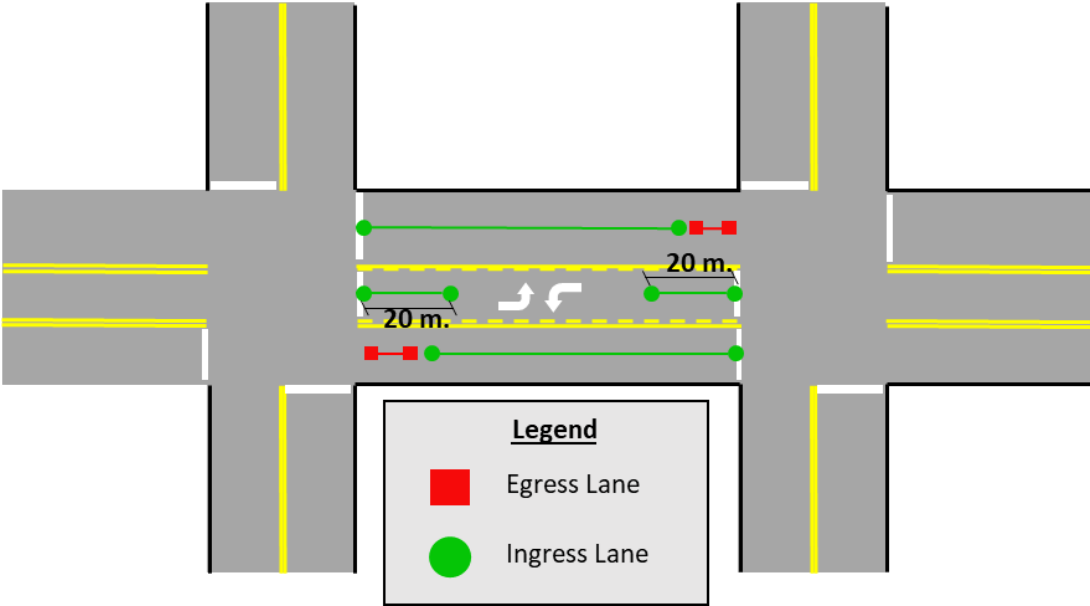
Figure 18: Two-way left-turn lanes Source: Athey Creek
